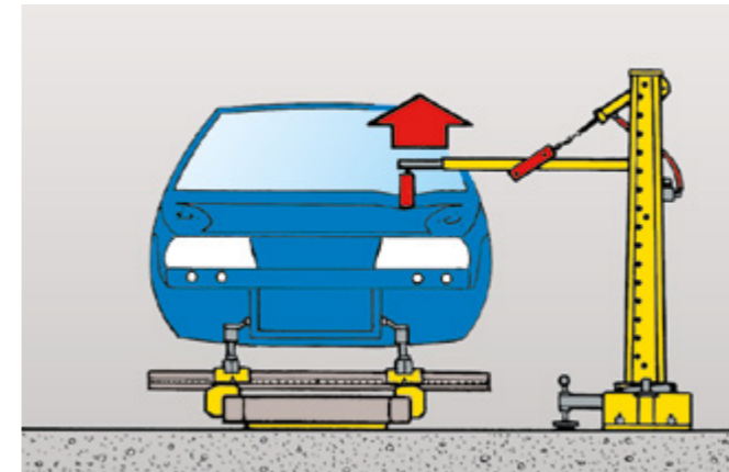
90BRATIR ● Device for vertical pull
